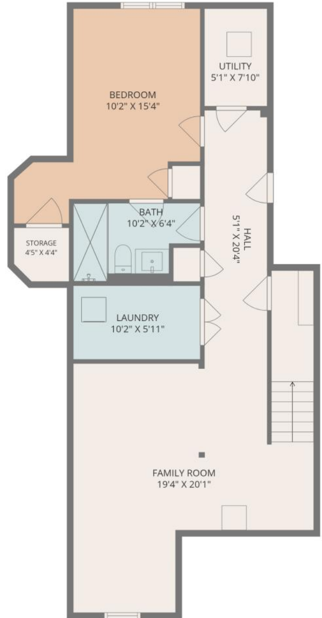
LOWER LEVEL
