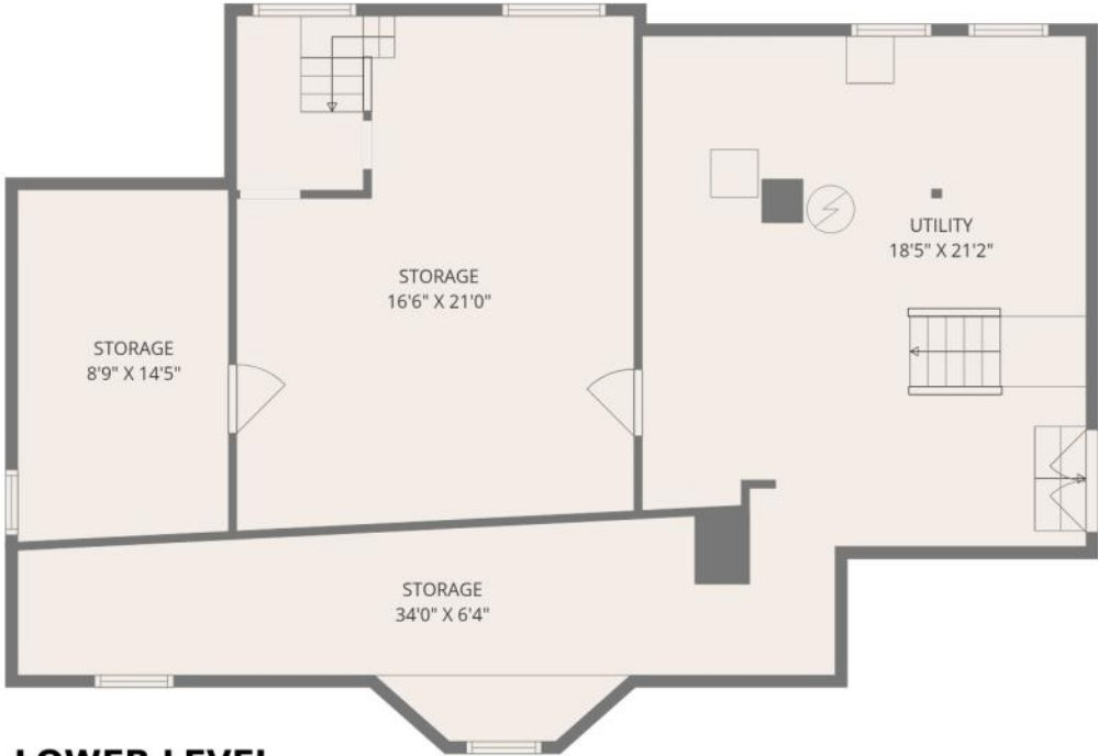
LOWER LEVEL
