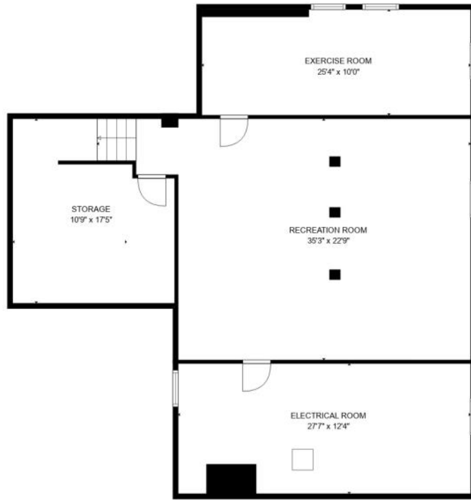
LOWER LEVEL
