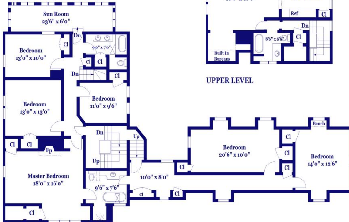
SECOND FLOOR
