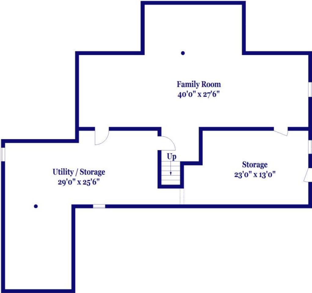
LOWER LEVEL
