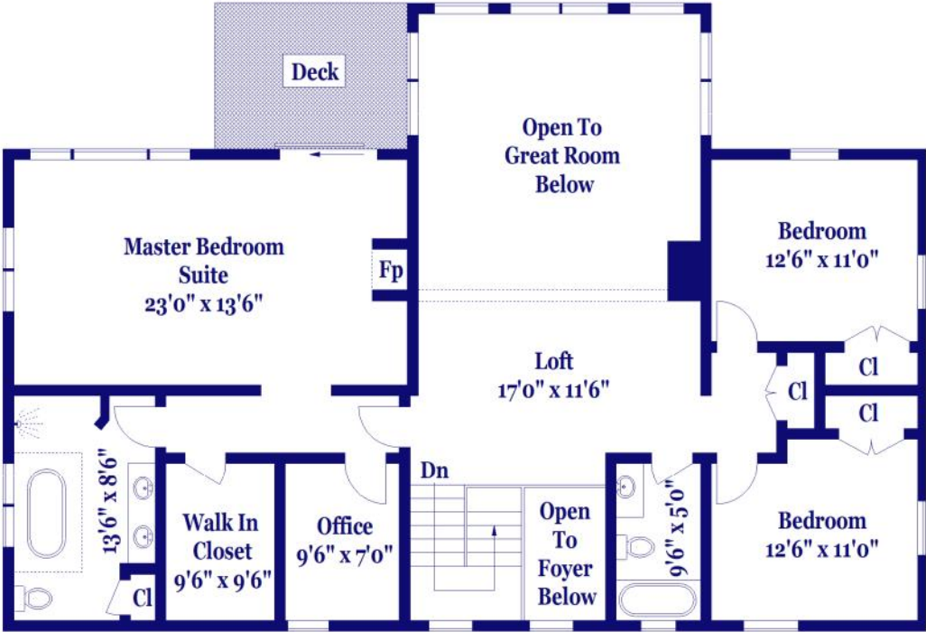
SECOND FLOOR
