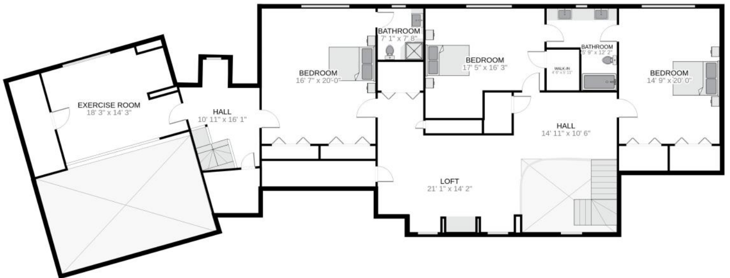
SECOND FLOOR
