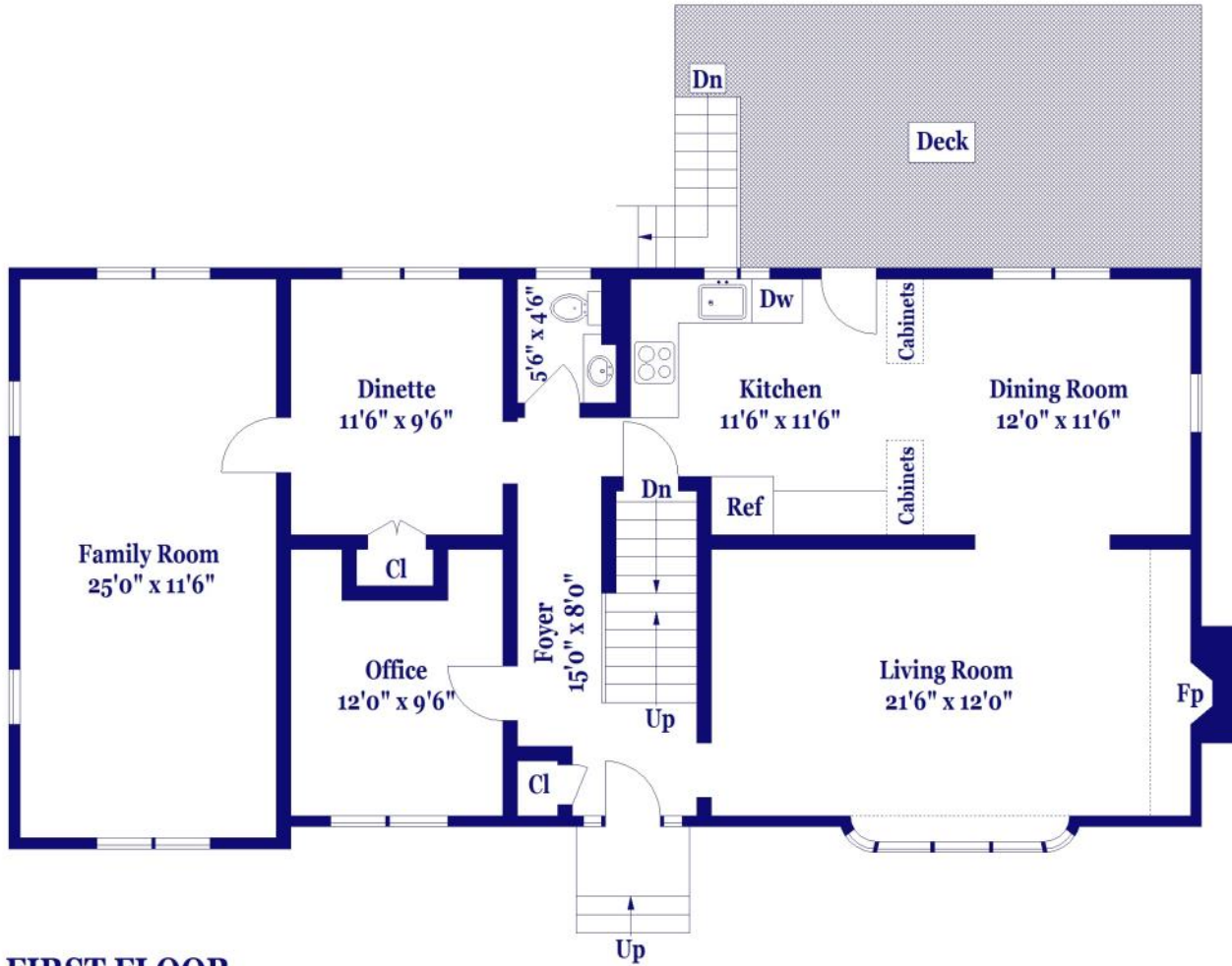
FIRST FLOOR
