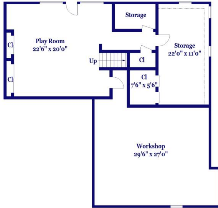
LOWER LEVEL
