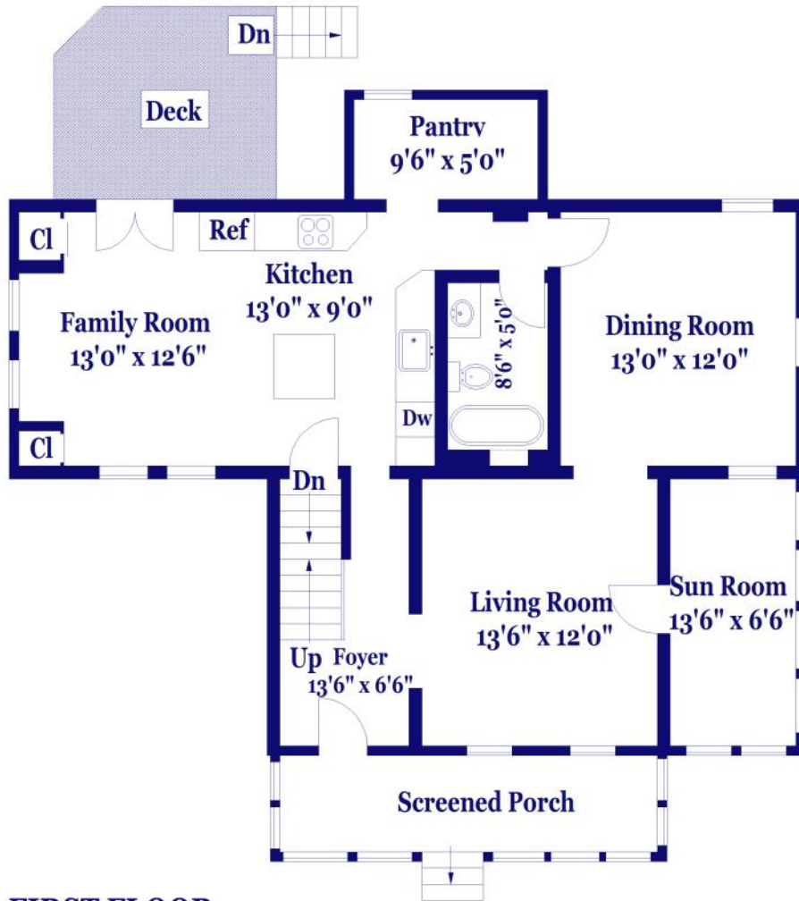
FIRST FLOOR
