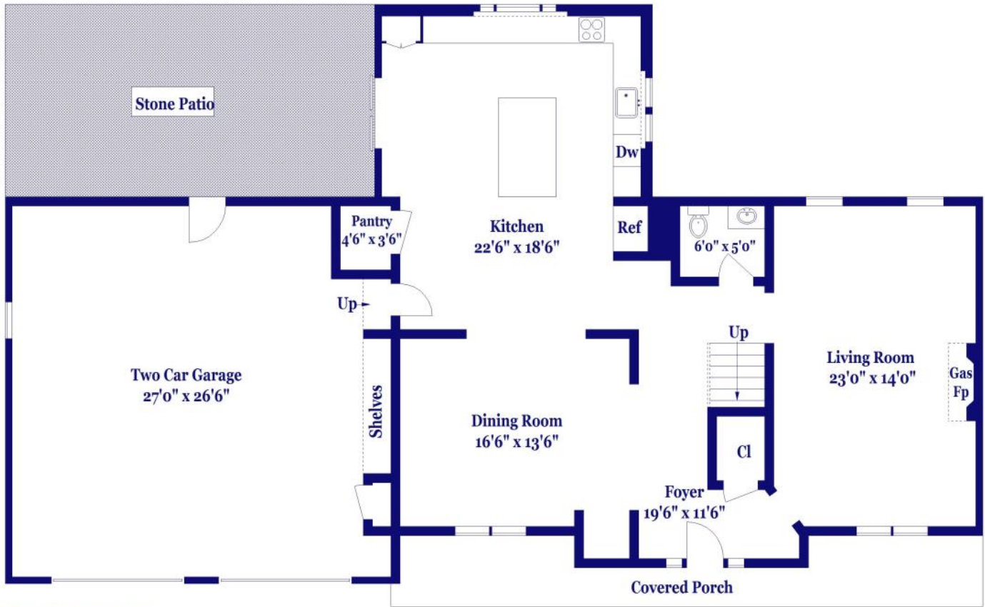
FIRST FLOOR
