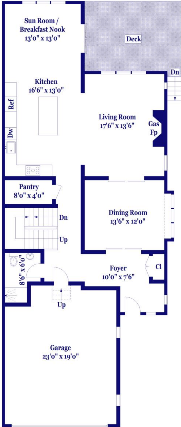
FIRST FLOOR
