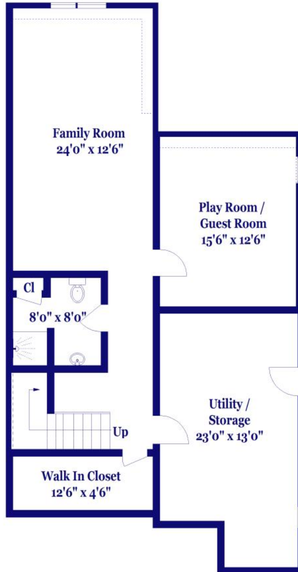
LOWER LEVEL
