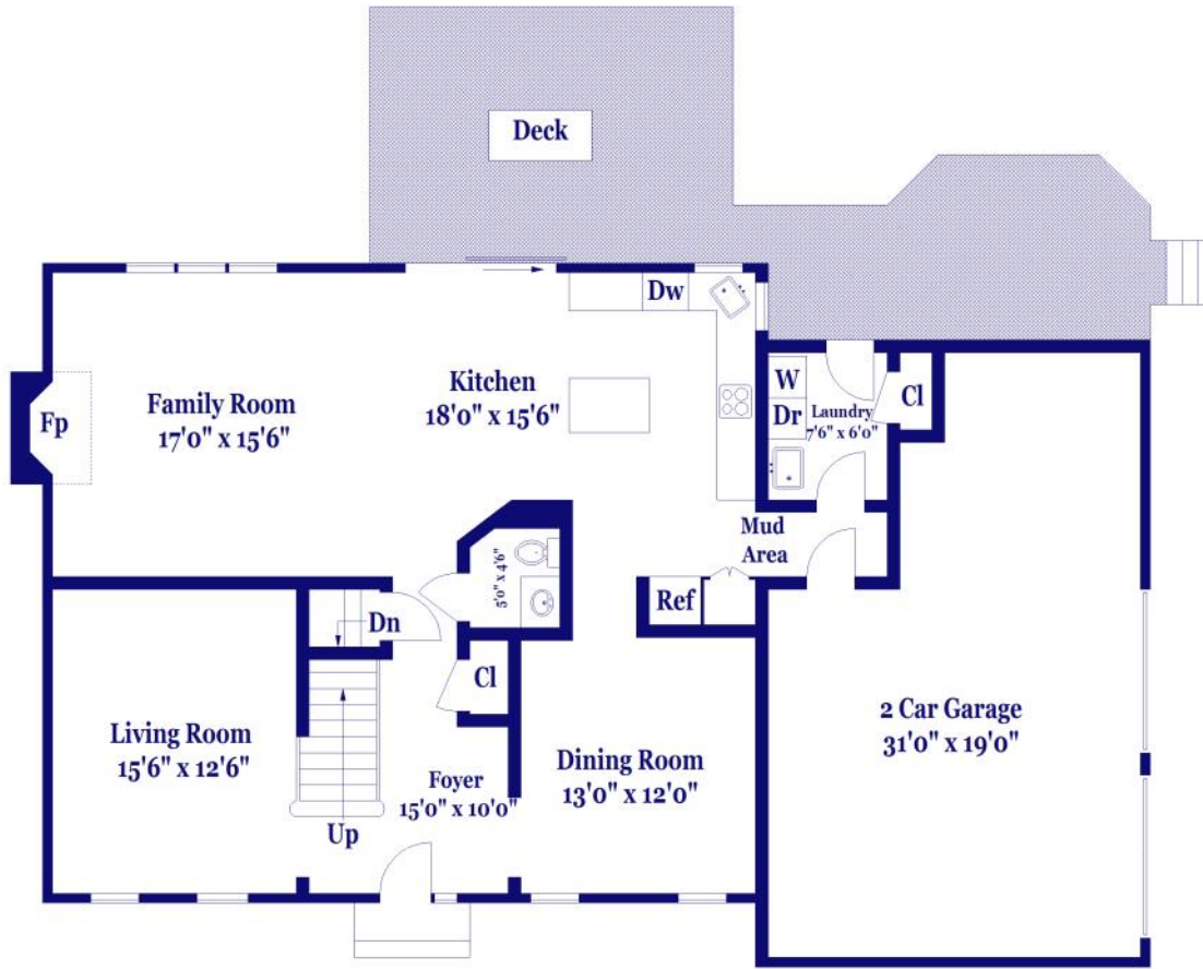
FIRST FLOOR
