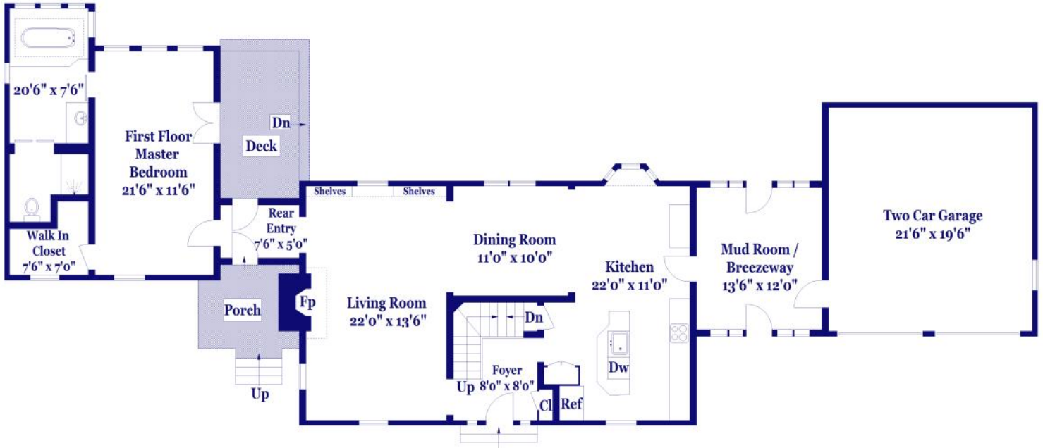
FIRST FLOOR
