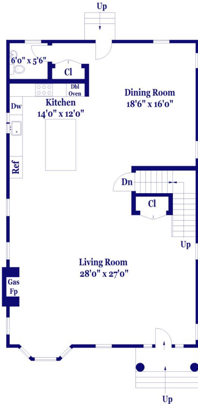
FIRST FLOOR
