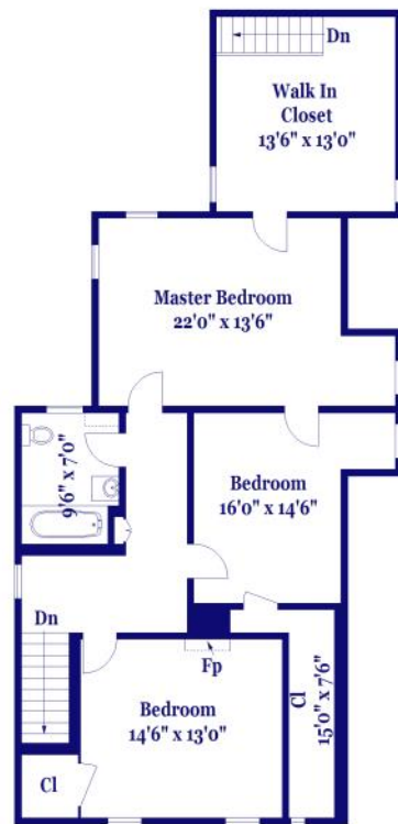
SECOND FLOOR
