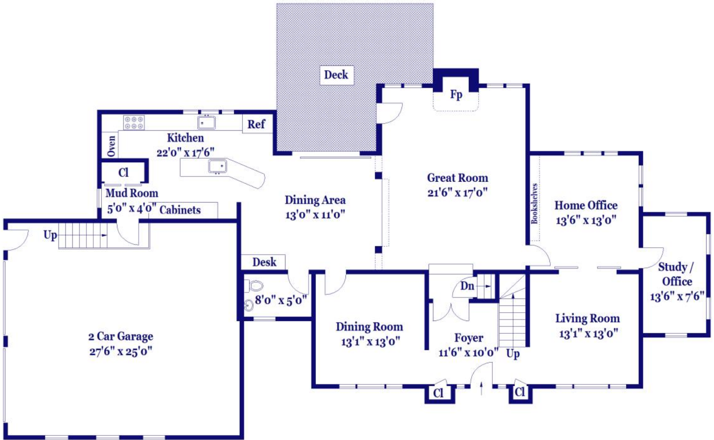
FIRST FLOOR
