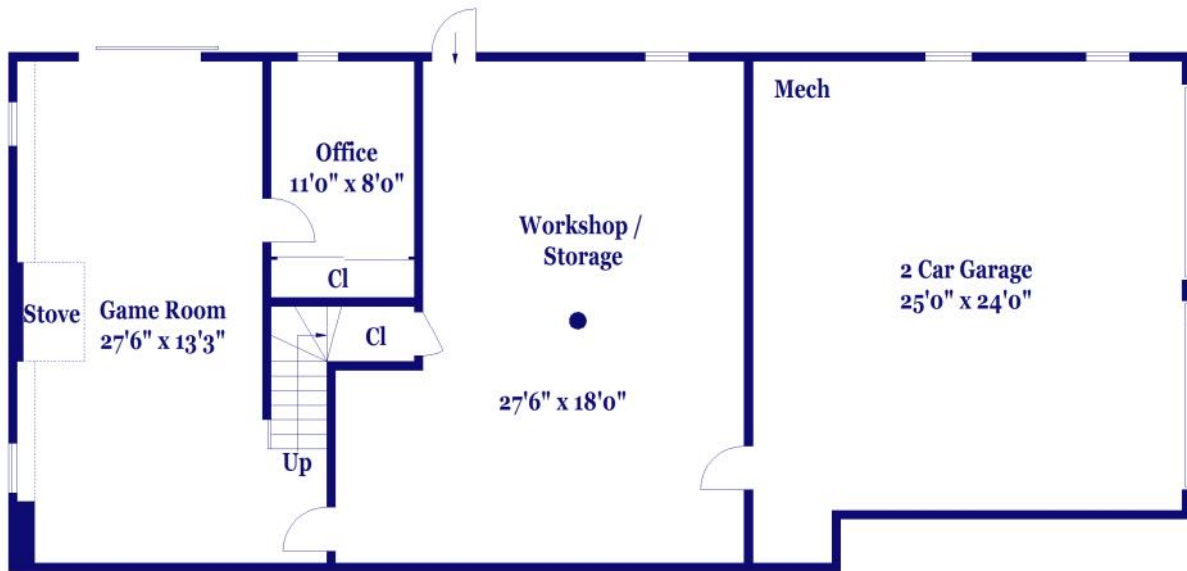
LOWER LEVEL
