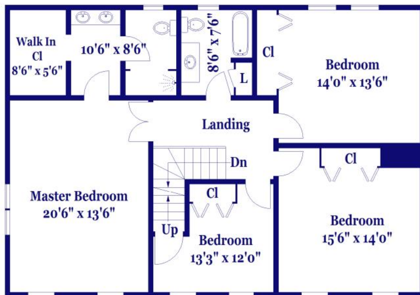
SECOND FLOOR
