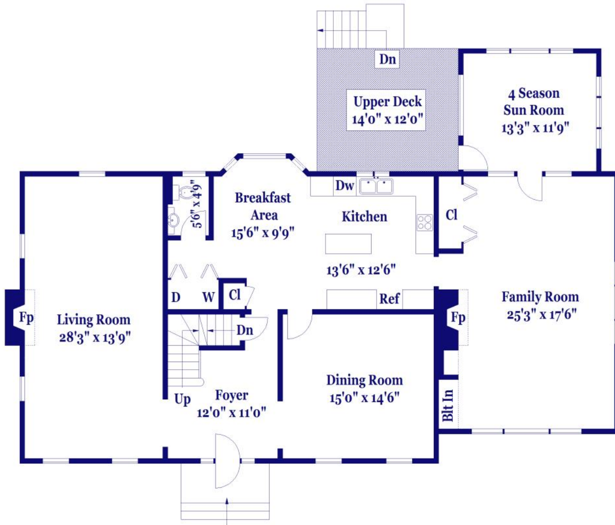
FIRST FLOOR
