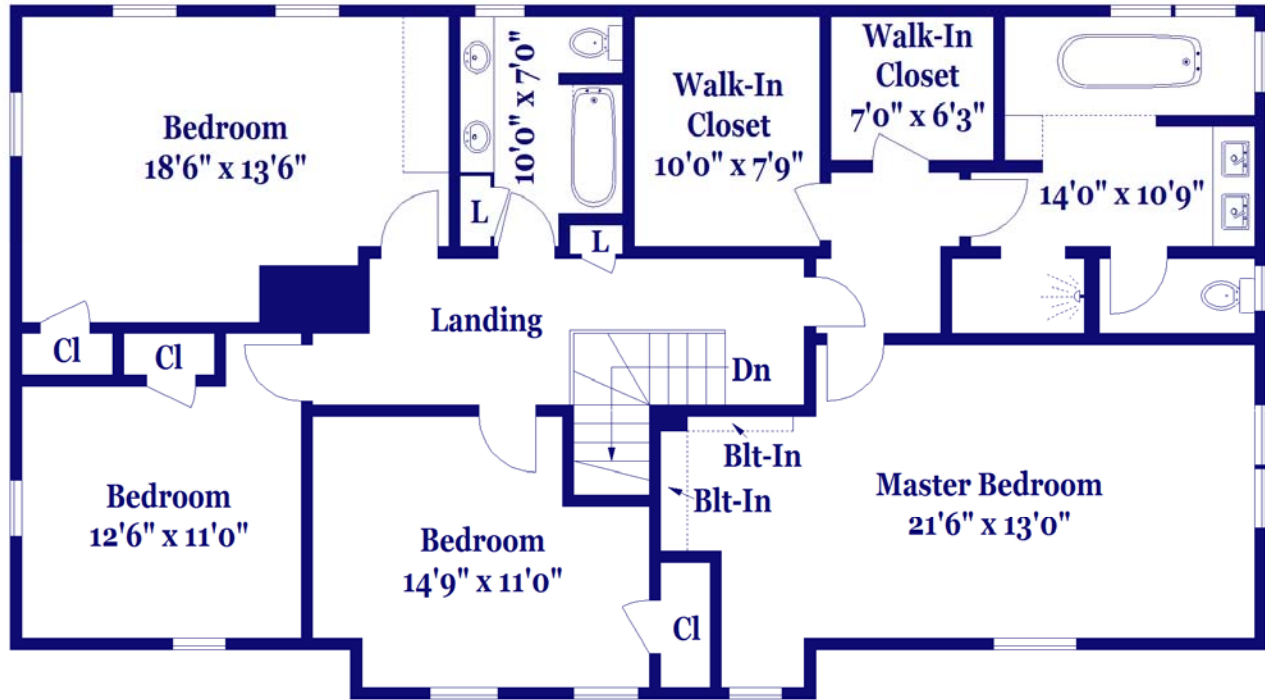
SECOND FLOOR
