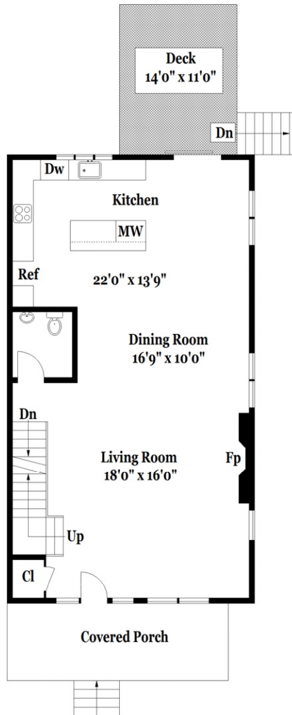
193 FIRST FLOOR "Similar To be Built"
