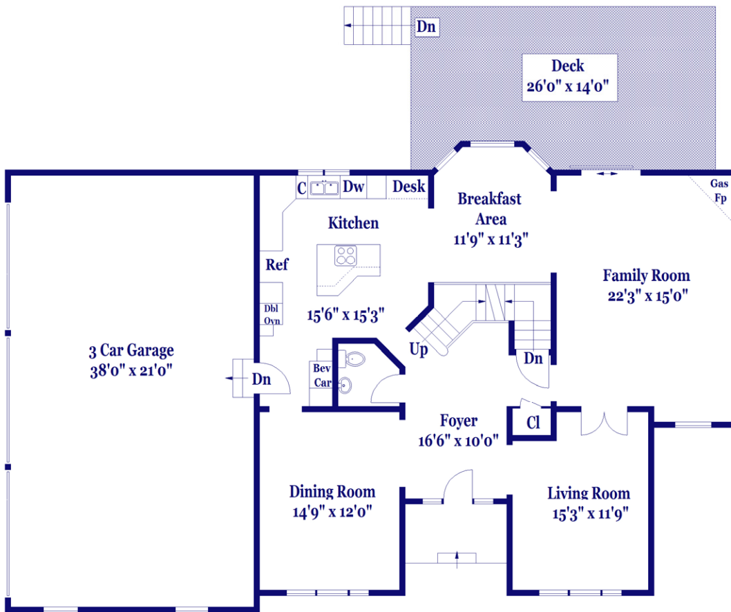
FIRST FLOOR
