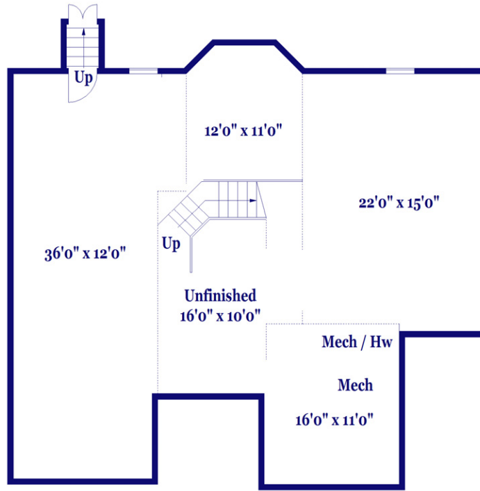
LOWER LEVEL
