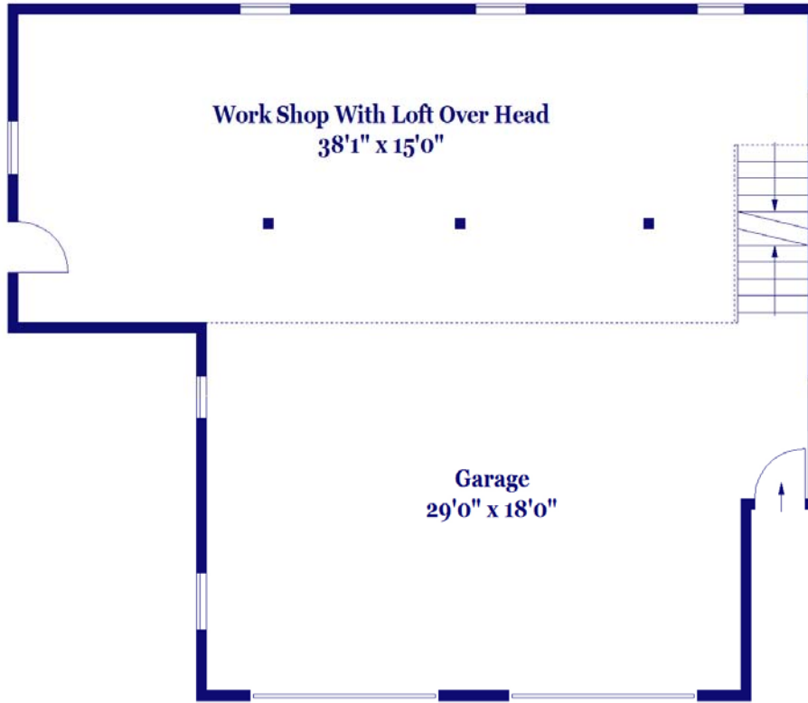
DETACHED GARAGE
