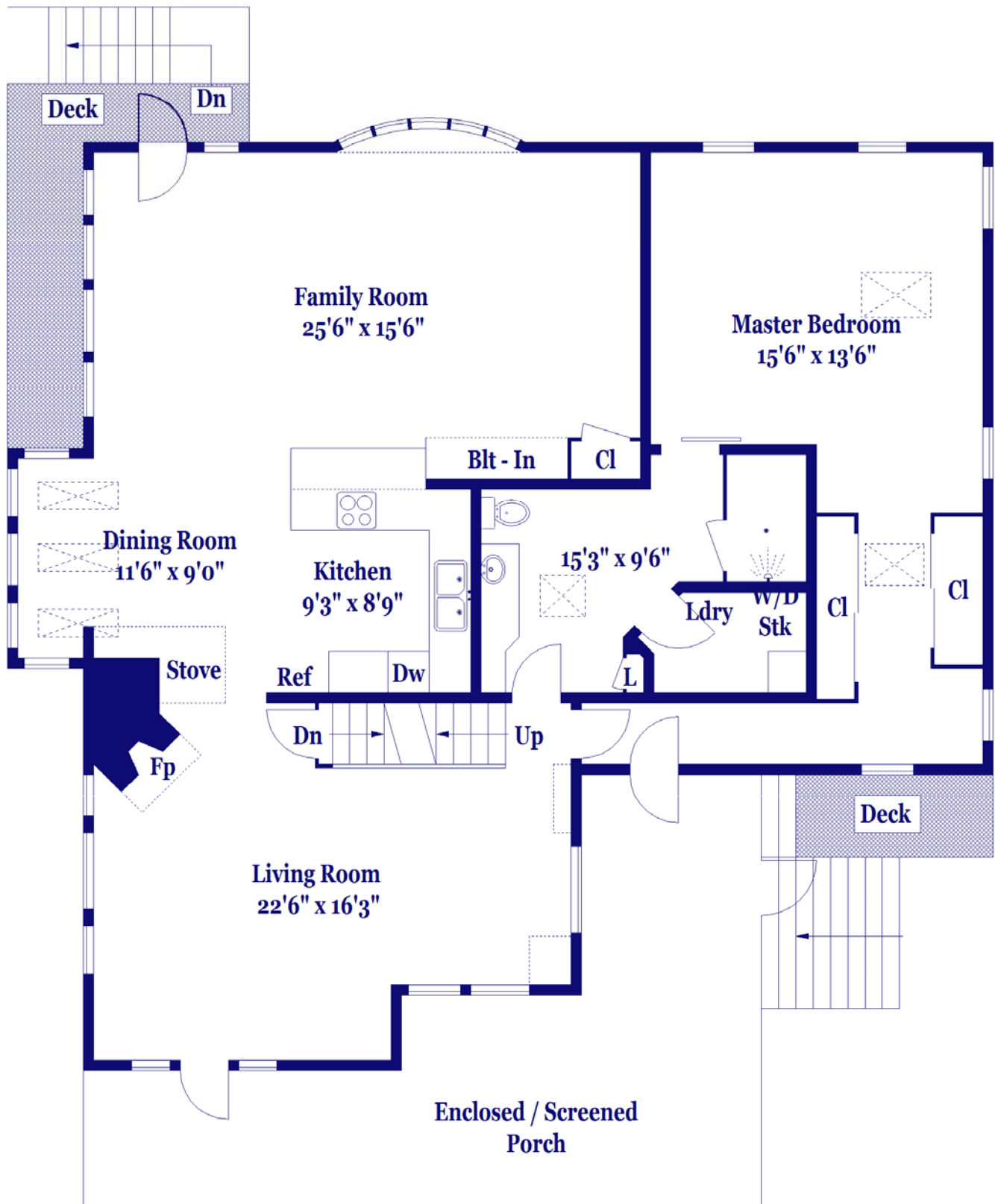
FIRST FLOOR
